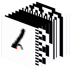
Input tensor with positional encoding
